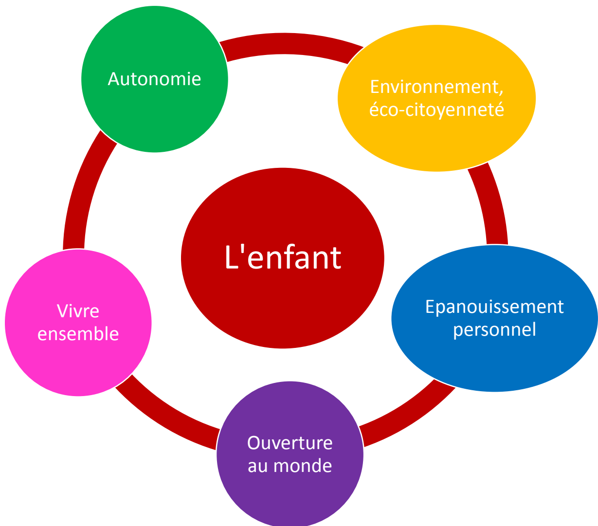
Figure 1 : intentions éducatives
